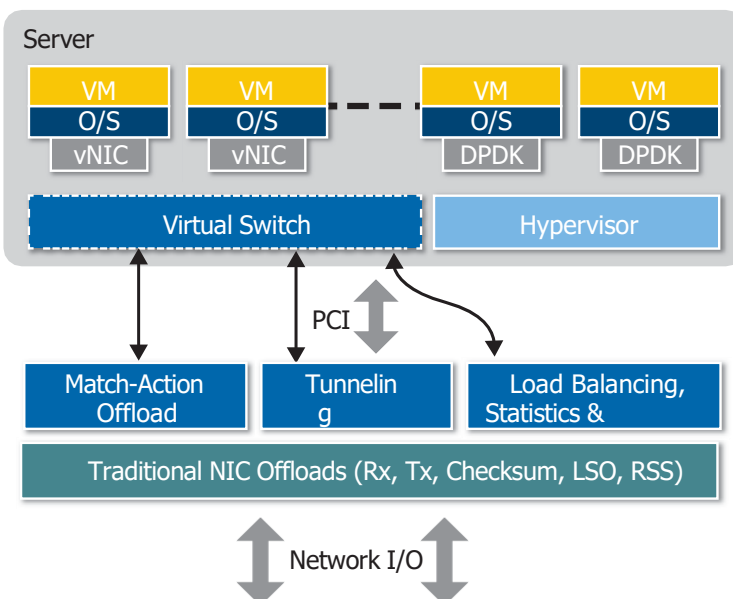
Agilio CX 2x25GbE SmartNIC Block Diagram
